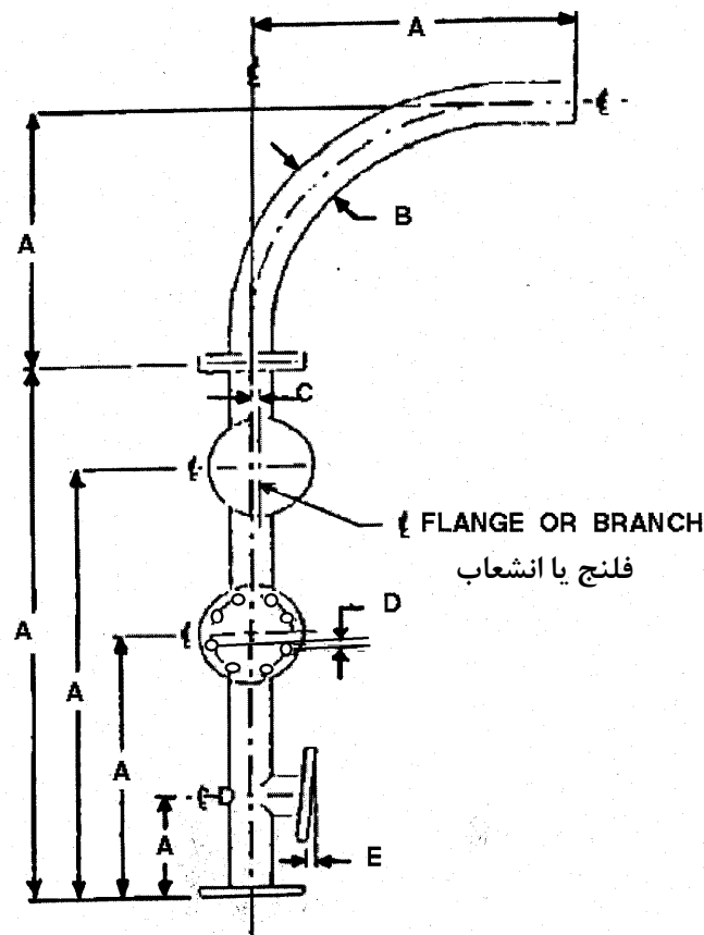
Fig. 1-DIMENSIONAL TOLERANCES FOR FABRICATED PIPEWORK
